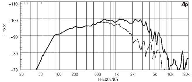
FREQUENCY RESPONSE CURVE OF 10W400 MADE ON 30 LIT. ENCLOSURE TUNED 55HZ INFREE FIELD (4PI) ENVIRONMENT. ENCLOSURE CLOSES THE REAR OF THE DRIVER. THE THIN LINE REPRESENTS 45 DEG. OFF AXIS FREQUENCY RESPONSE
