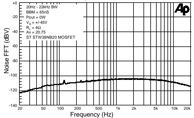
A-Weighted Noise FFT
